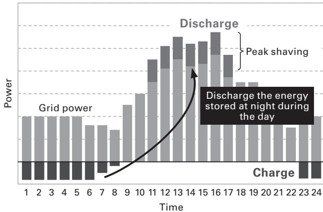
Fig. 4 Schedule-based charge/discharge control illustrated
