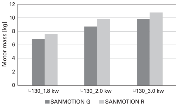
Fig. 11 Comparison of medium-inertia motor mass (Without holding brake)
