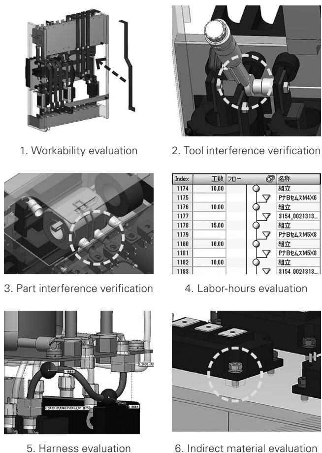
Fig. 6 Examples of evaluation performed in the VPS
