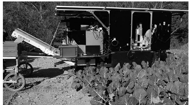
Fig. 1 Broccoli harvesting robot
