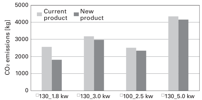
Fig. 12 Comparison of servo motor CO 2 emissions
