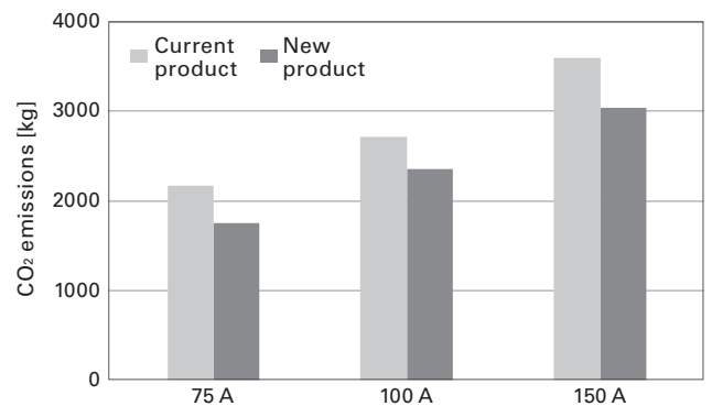
Fig. 13 Comparison of servo amplifier CO 2 emissions
