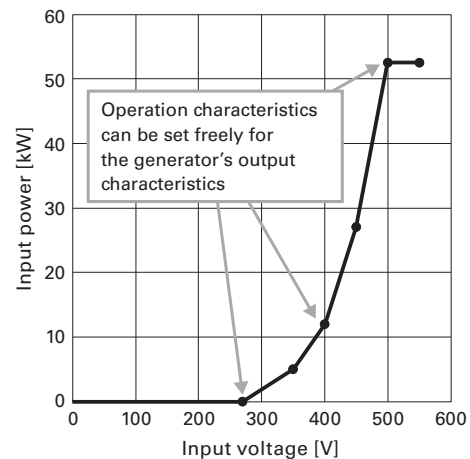
Fig. 3 Generator power curve settings illustrated
