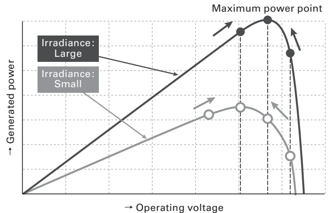
Fig. 2 MPPT control illustrated
