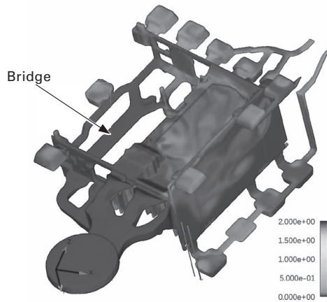
Fig. 16 Die casting fluid analysis (with bridge)
