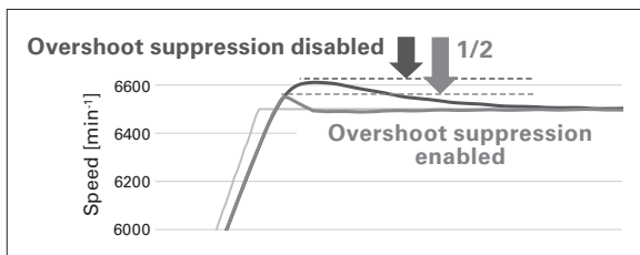
Fig. 7 Overshoot suppression characteristics
