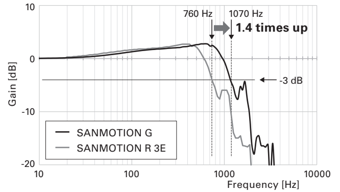
Fig. 5 Comparison of closed-loop frequency response for the speed control system
