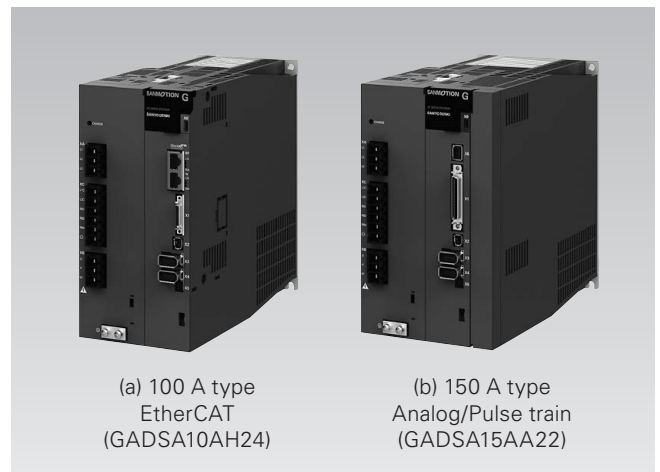
Fig. 2 Servo amplifier appearance
