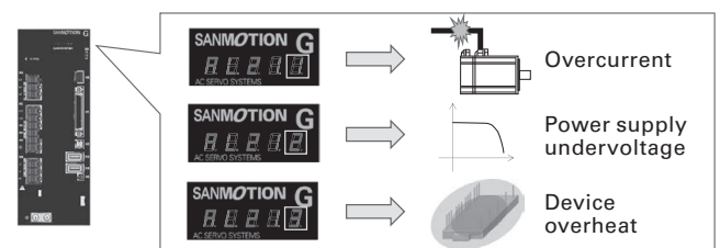
Fig. 9 Divided power device errors
