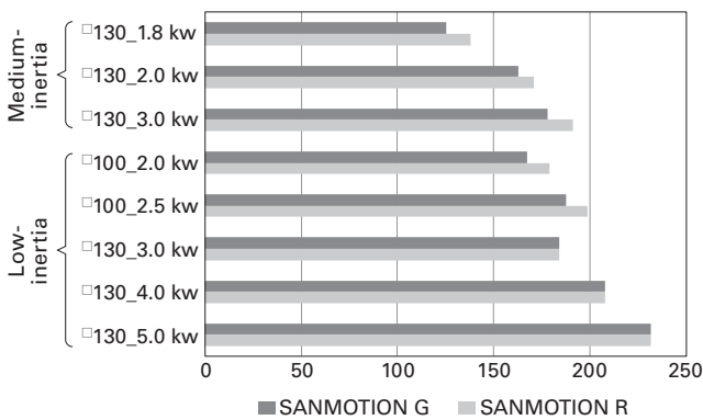
Fig. 10 Comparison of motor length (Without holding brake)
