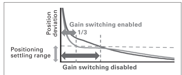
Fig. 6 Positioning settling characteristics
