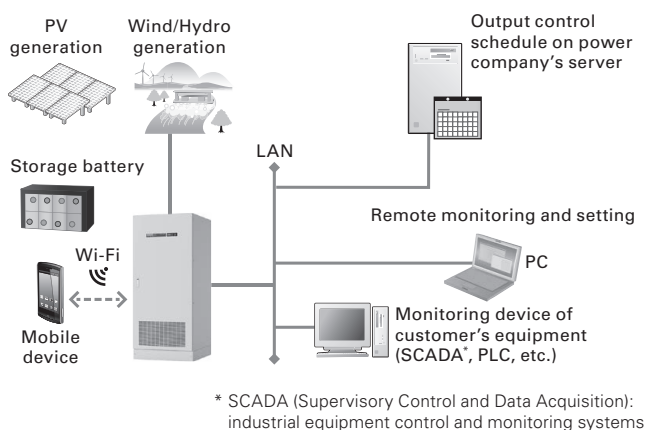
Fig. 13 The SANUPS W83A system configuration example
