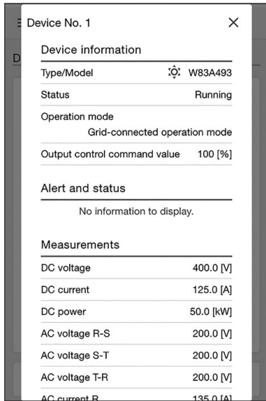
Fig. 8 Unit status and measurement data screen
