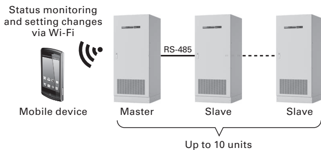
Fig. 5 Illustrative image of the connection between a mobile device and the SANUPS W83A
