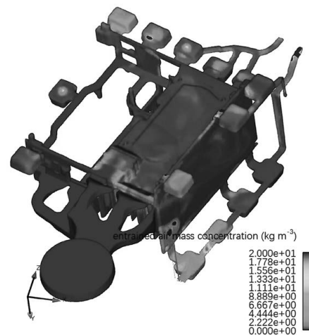
Fig. 15 Die casting fluid analysis (initial phase of development)
