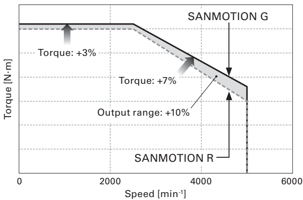
Fig. 4 Comparison of T-N characteristics of medium-inertia motors
