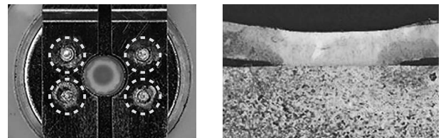
Fig. 9 Weld mark and cross-section
