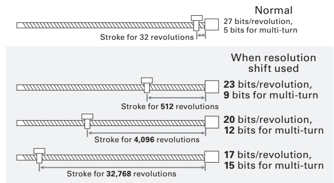
Fig. 8 Encoder resolution shifting illustrations
