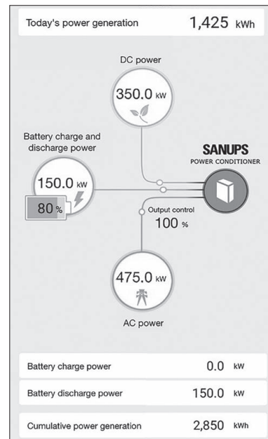
Fig. 6 Dashboard screen
