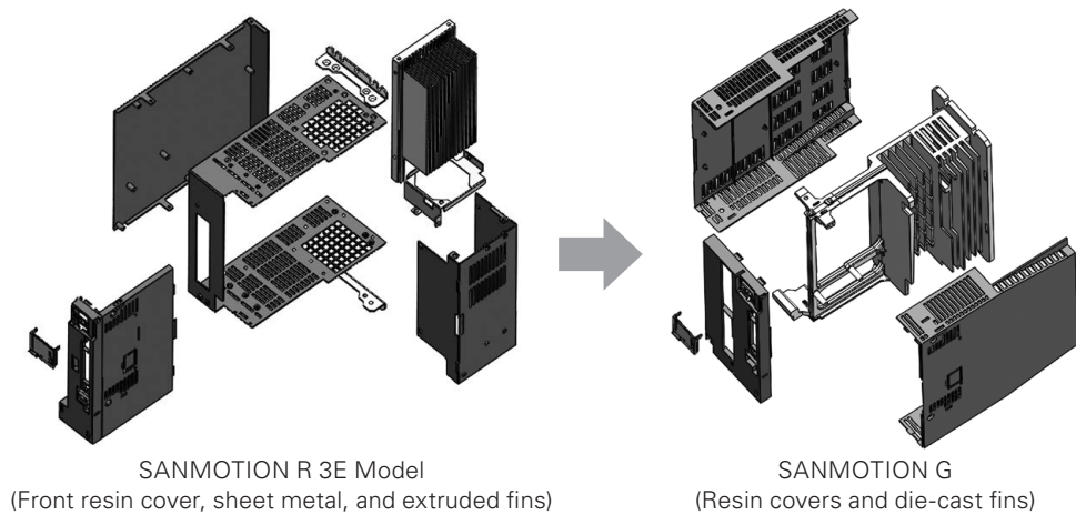
Fig. 3 Housings of current and new products
