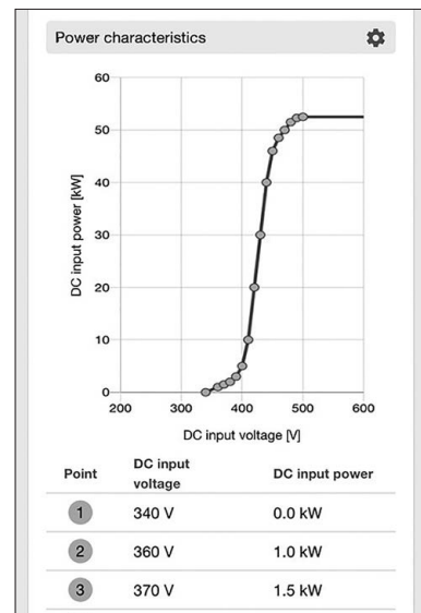
Fig. 11 Generator power curve setting screen
